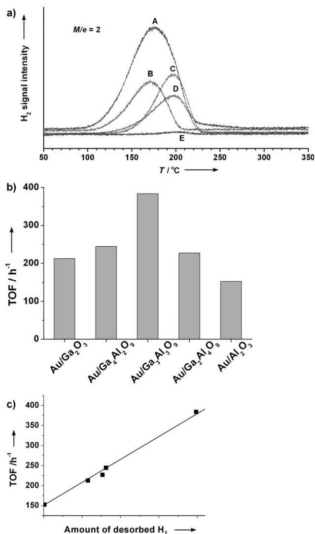
Figure 1. a) TPSR diagram of 2-propanol on various gold catalysts ( H_2 mass intensity): Au/Ga_3Al_3O_9 (A), Au/Ga_4Al_2O_9 (B), Au/Ga_2Al_4O_9 (C), Au/Ga_2O_3 (D), and Au/Al_2O_3 (E); the mass/charge ratio ( M/e ) = 2. b) TOF for the aerobic oxidation of benzyl alcohol using gold supported on different mixed oxides, Ga_xAl_{6-x}O_9 ( x=0, 2, 3, 4, 6 ), as catalysts (measured at t=1 h). Conditions: 90^\circ C , catalyst (100 mg), benzyl alcohol (3.85 mmol), O_2 bubbling rate: 20\text{ mL min}^{-1} . Trace amounts of byproducts were detected. c) Correlation between the amount of desorbed H_2 and the specific oxidation rate of benzyl alcohol using Au/Ga_xAl_{6-x}O_9 ( x=0, 2, 3, 4, 6 ) catalysts. The amount of desorbed H_2 was determined from the relative peak area of the H_2 mass signal.
